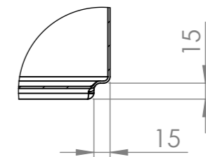
DETAIL C SCALE 1 : 5
